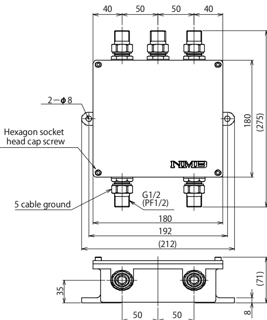
Parts No. : SB-310-4-B*
