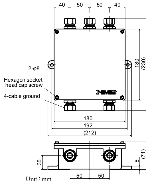
Parts No. : SB-310-4-A*
