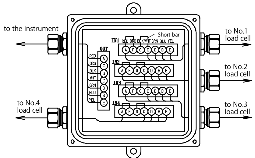
Parts No. : SB-310-4-A*
