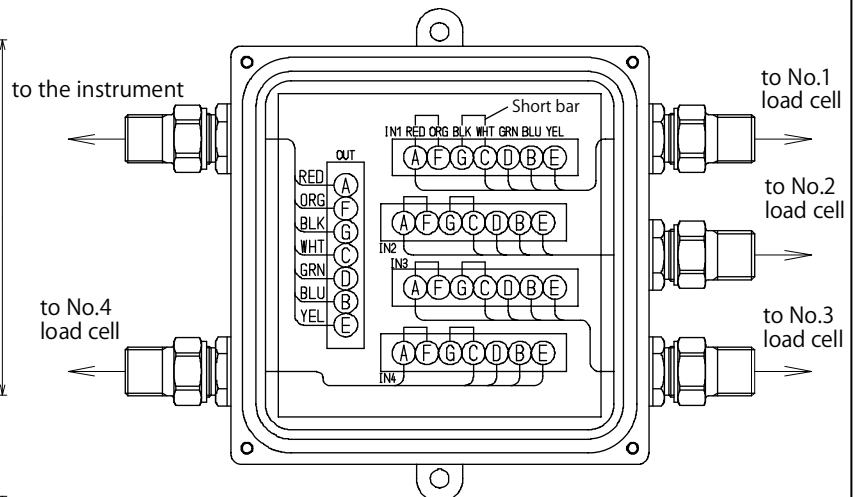
Parts No. : SB-310-4-A*
